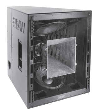
EAW KF750F 3 pásma full range, 2×12" dipolar array + 10" horn + 2", 1 200 W/103 dB + 400 W/109 dB + 200 W/116 dB, triamp
